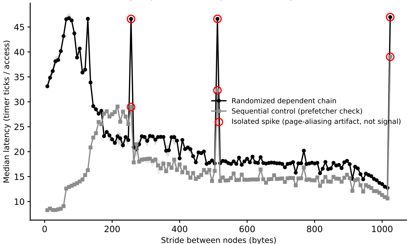
hazel_broadwell: line-size sweep (dependent pointer chase), footprint=512 KiB (Phase I timing-only, level boundary=262144B, single-curve method)
