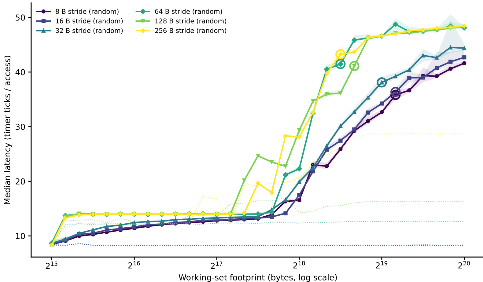
hazel_broadwell: line-size family of curves (dependent pointer chase) (Phase I timing-only, level boundary=262144B window=[32768,1048576])
