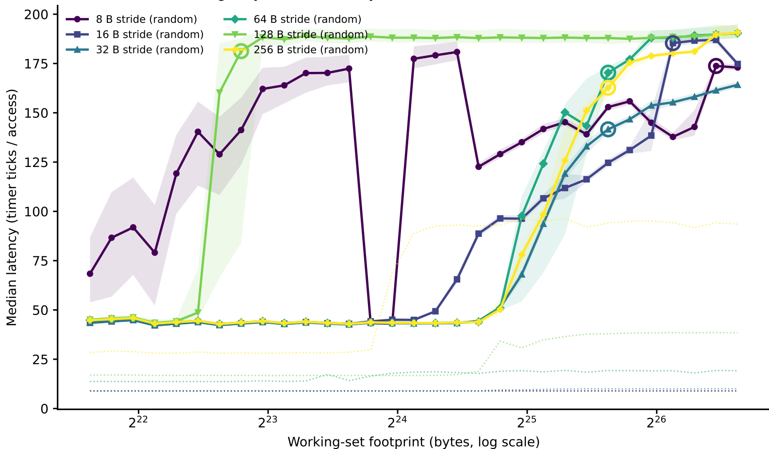
hazel_broadwell/line_size_rerun: line-size family of curves (dependent pointer chase) (Phase I timing-only, level boundary=25874000B window=[3234250,103496000])
