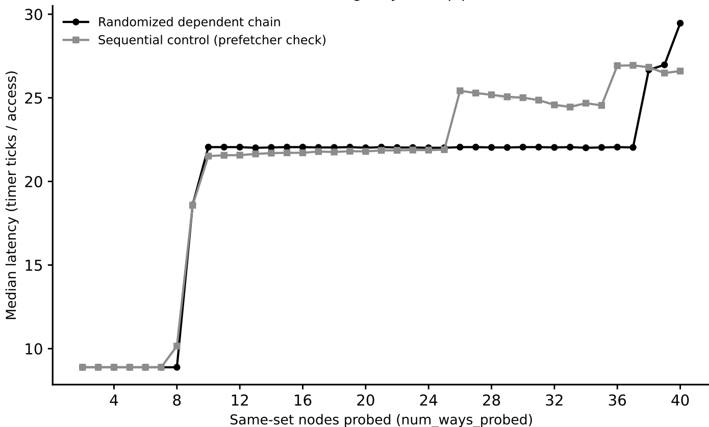
hazel_broadwell/phase1_v2: associativity sweep, L1 (stride=32 KiB) (Phase I timing-only, auto pipeline)
