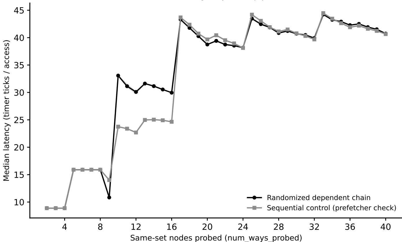
hazel_broadwell/phase1_v2: associativity sweep, L2 (stride=256 KiB) (Phase I timing-only, auto pipeline)
