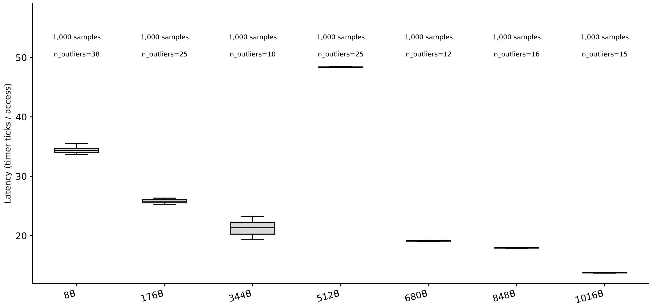
hazel_broadwell/phase1_v2: line-size box plots, random pattern (whiskers = p5/p95) (Phase I timing-only, level boundary=262144B, single-curve method)
