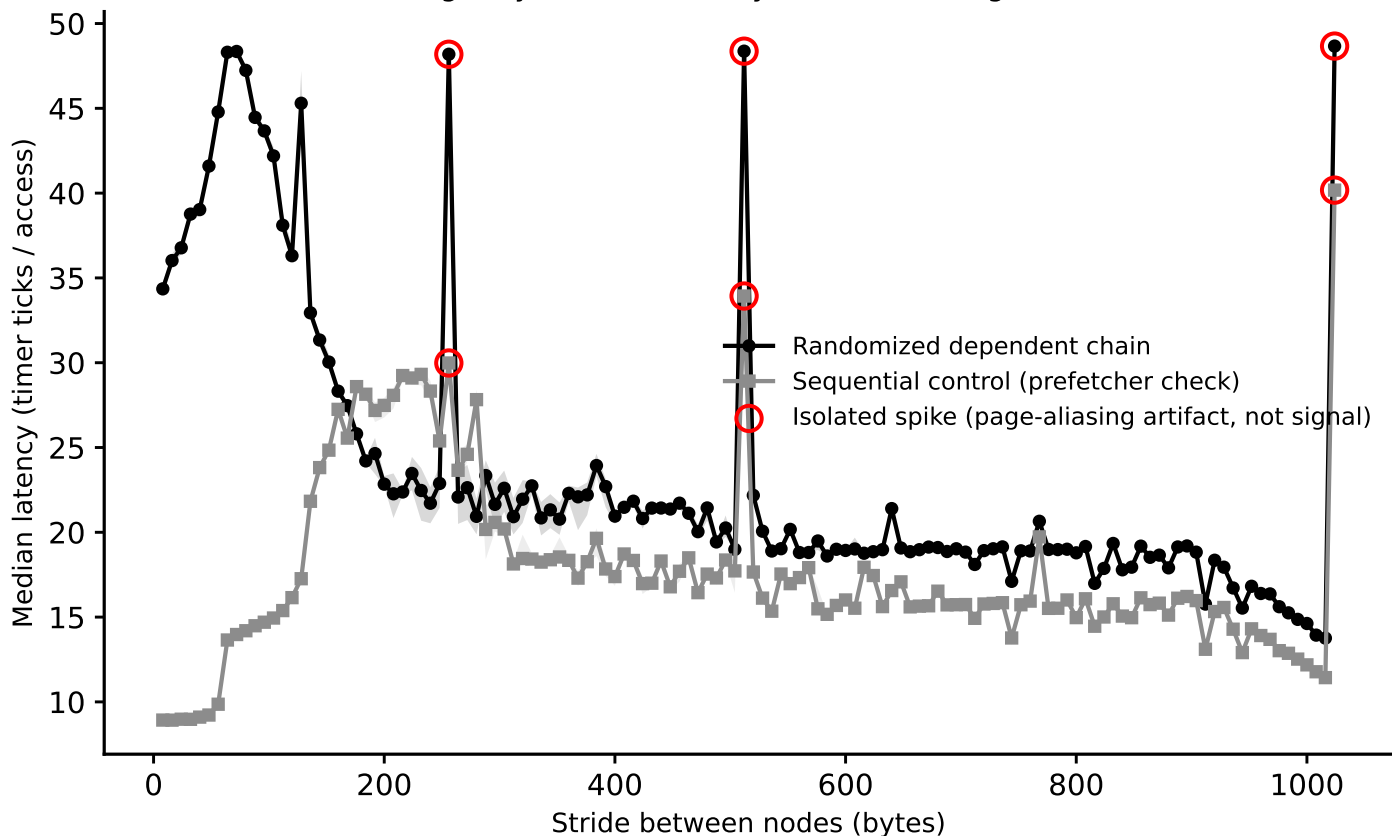
hazel_broadwell/phase1_v2: line-size sweep (dependent pointer chase), footprint=512 KiB (Phase I timing-only, level boundary=262144B, single-curve method)
