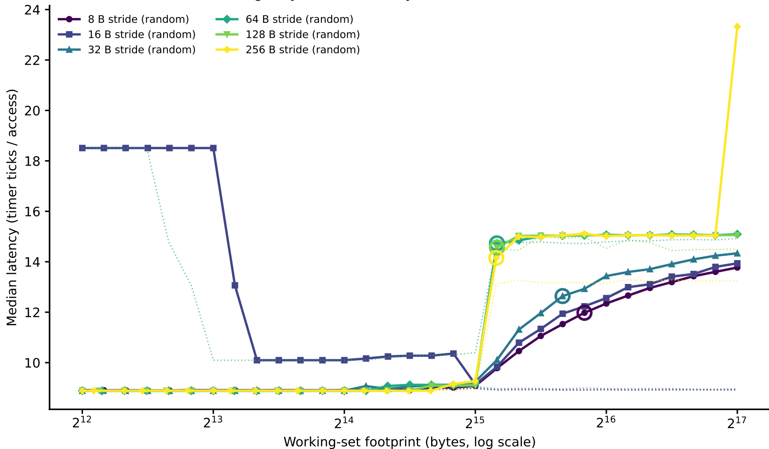
hazel_broadwell/phase1_v2: line-size family of curves (dependent pointer chase) (Phase I timing-only, level boundary=32768B window=[4096,131072])
