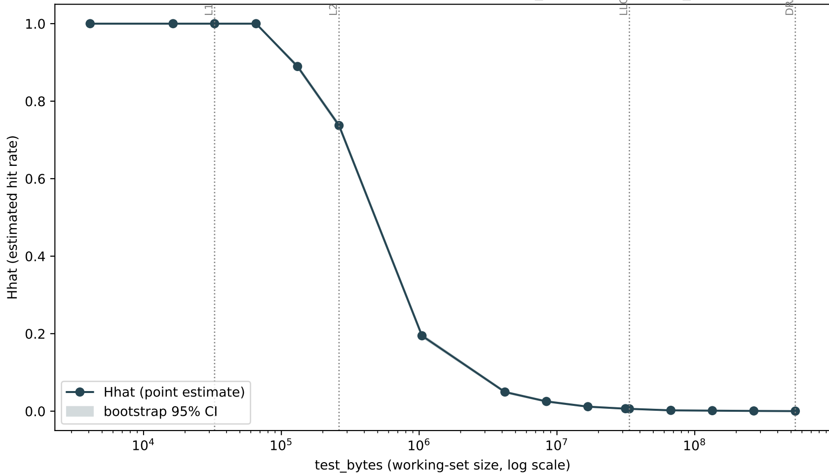
Software-only Hhat vs. working-set size (hazel_broadwell/phase1_v2)
