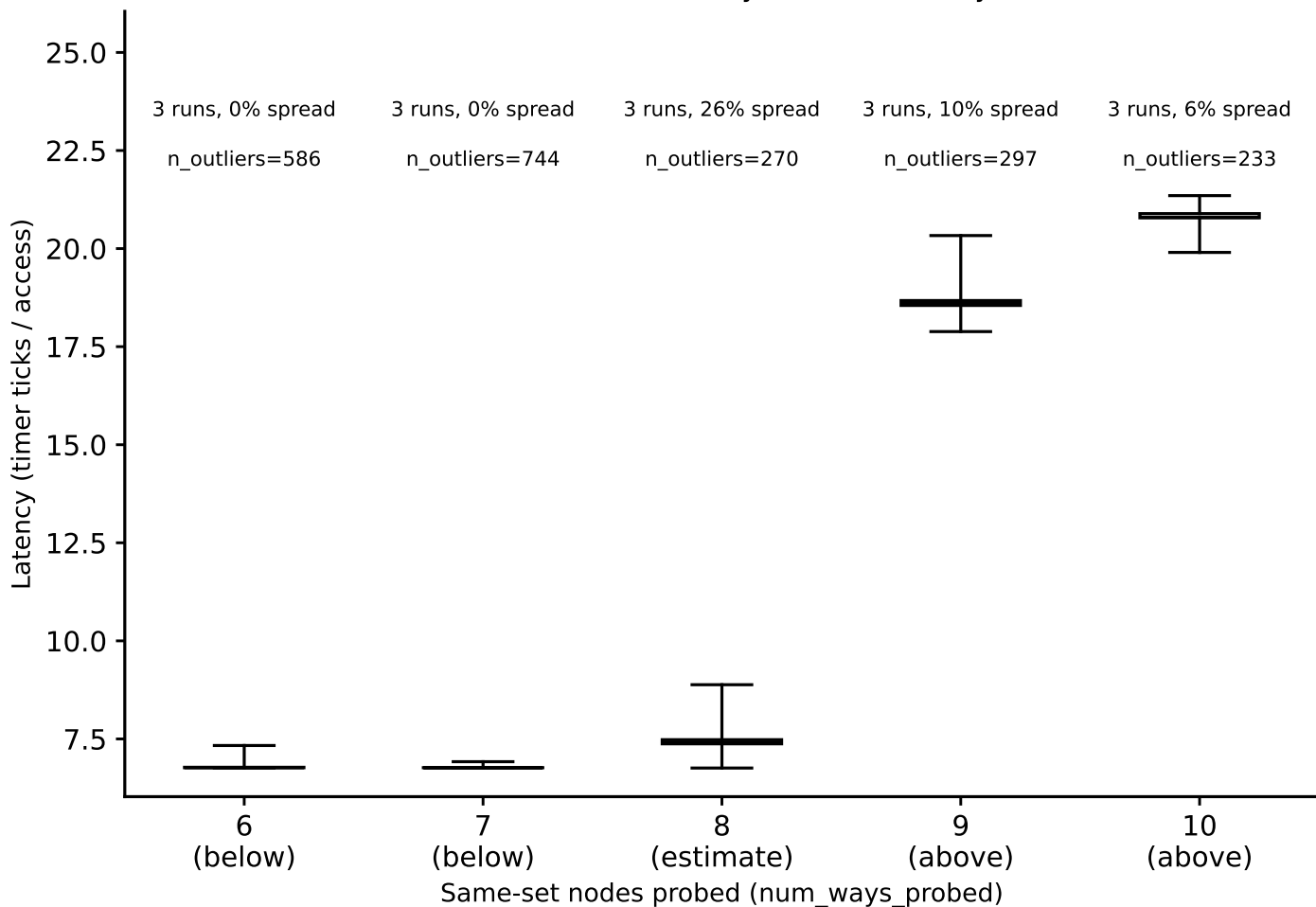
hazel_cascadelake: associativity box plots, L1, random pattern (whiskers = p5/p95) (Phase I timing-only, auto pipeline) detected associativity estimate: 8-way
