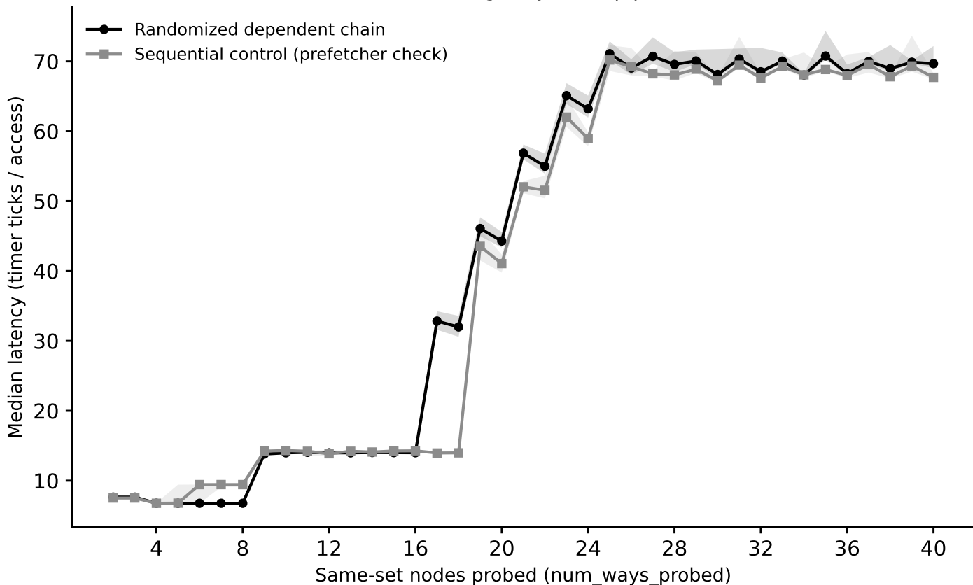
hazel_cascadelake: associativity sweep, L2 (stride=1 MiB) (Phase I timing-only, auto pipeline)
