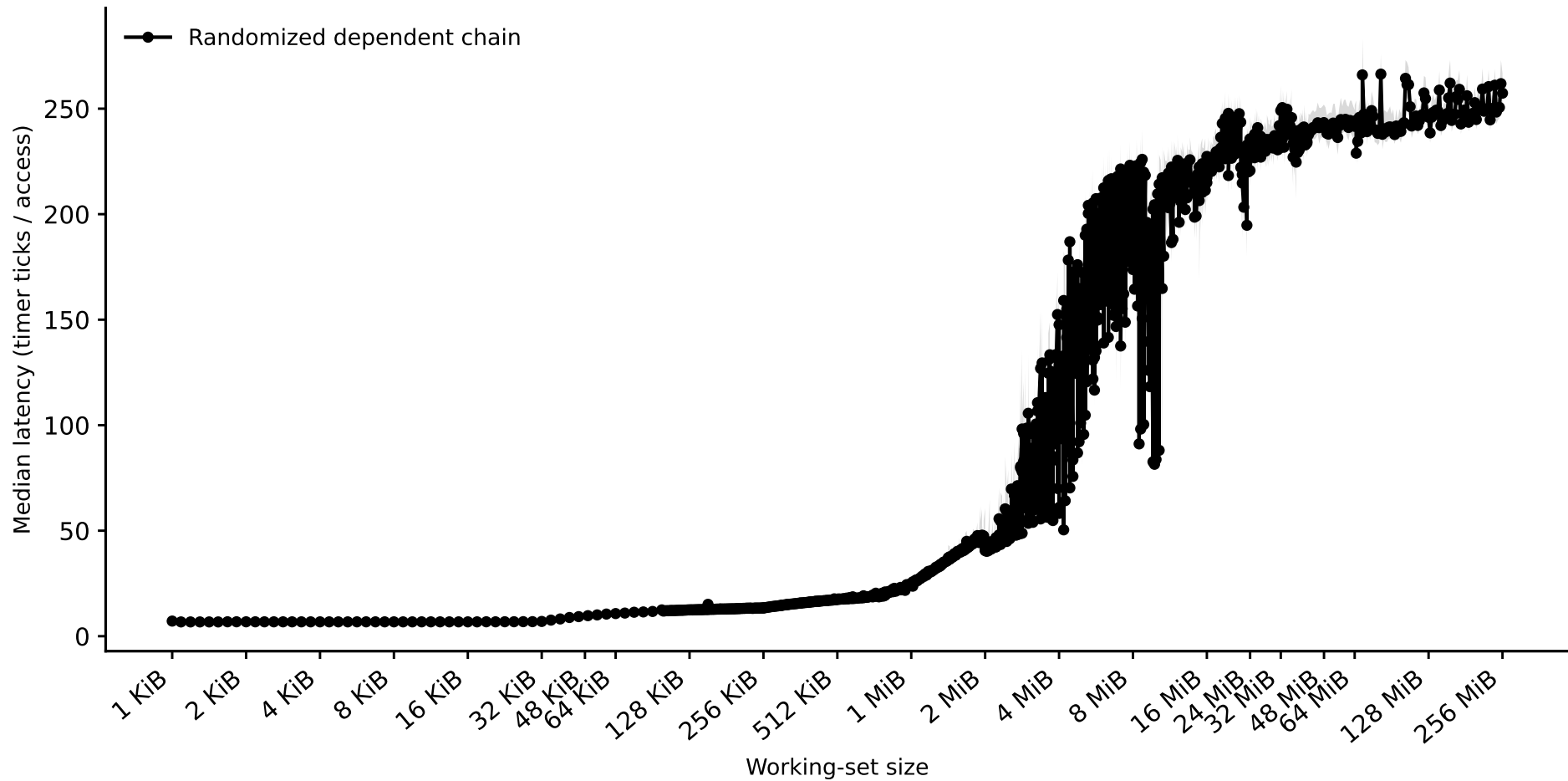
hazel_cascadelake: capacity sweep (dependent pointer chase) (Phase I timing-only, auto pipeline)
