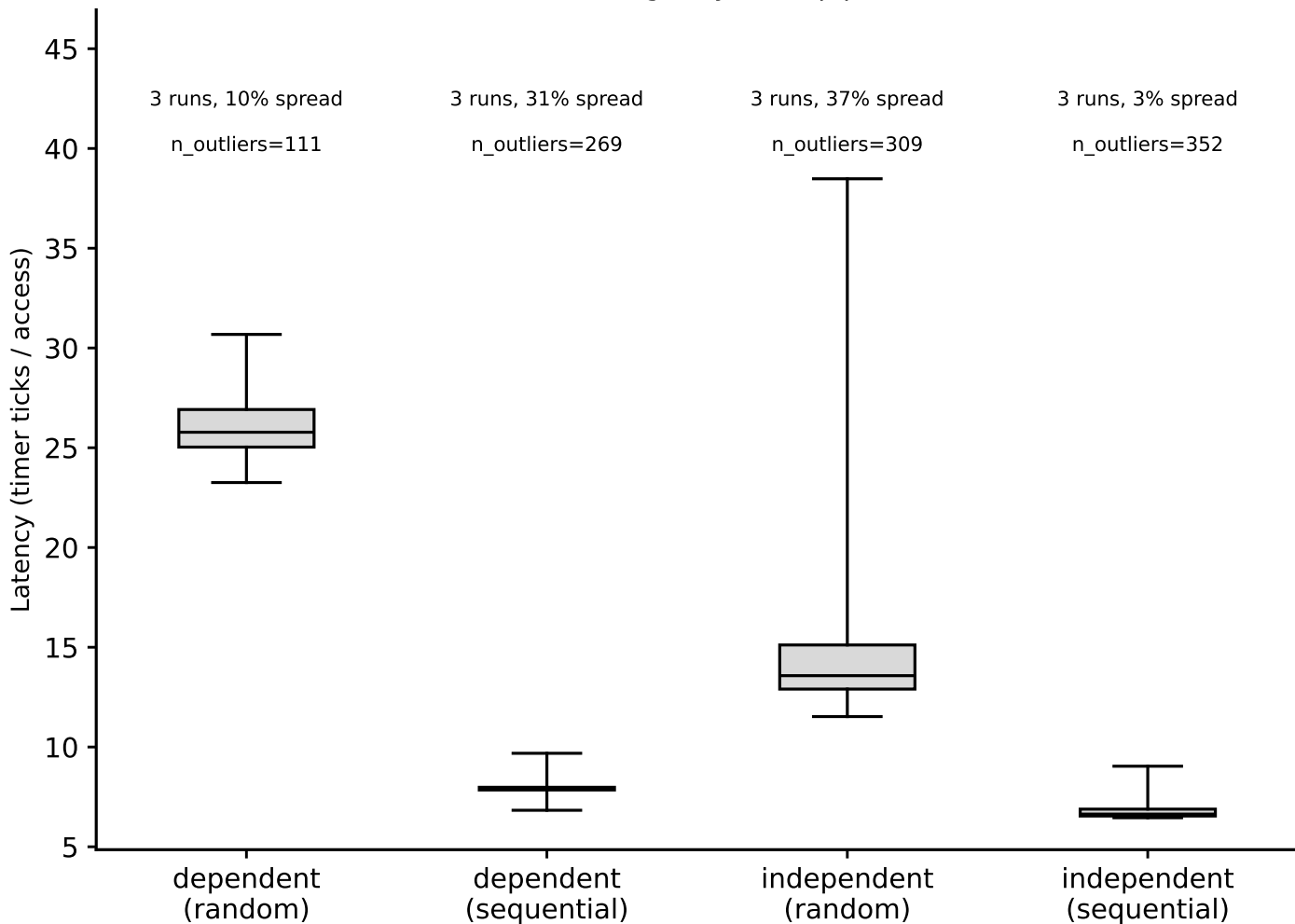
hazel_cascadelake: hit-latency box plots, L2 (footprint=1 MiB) (Phase I timing-only, auto pipeline)
