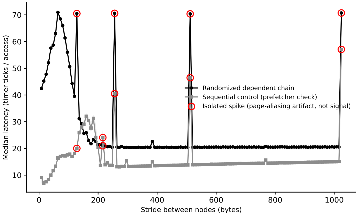
hazel_cascadelake: line-size sweep (dependent pointer chase), footprint=2 MiB (Phase I timing-only, level boundary=1048576B, single-curve method)
