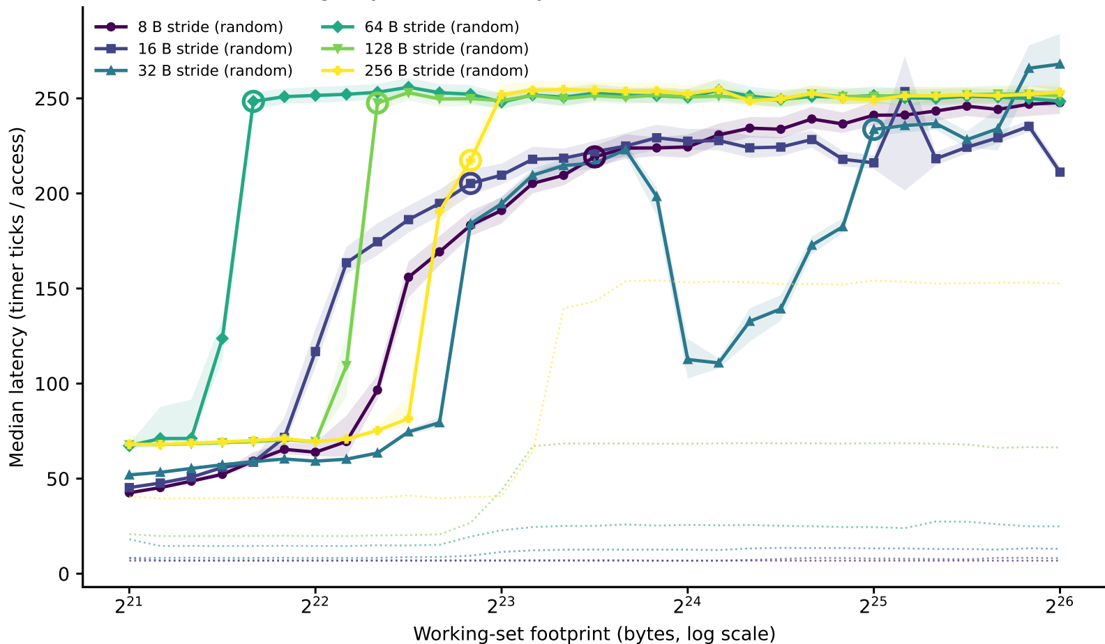
hazel_cascadelake: line-size family of curves (dependent pointer chase) (Phase I timing-only, level boundary=16777216B window=[2097152,67108864])
