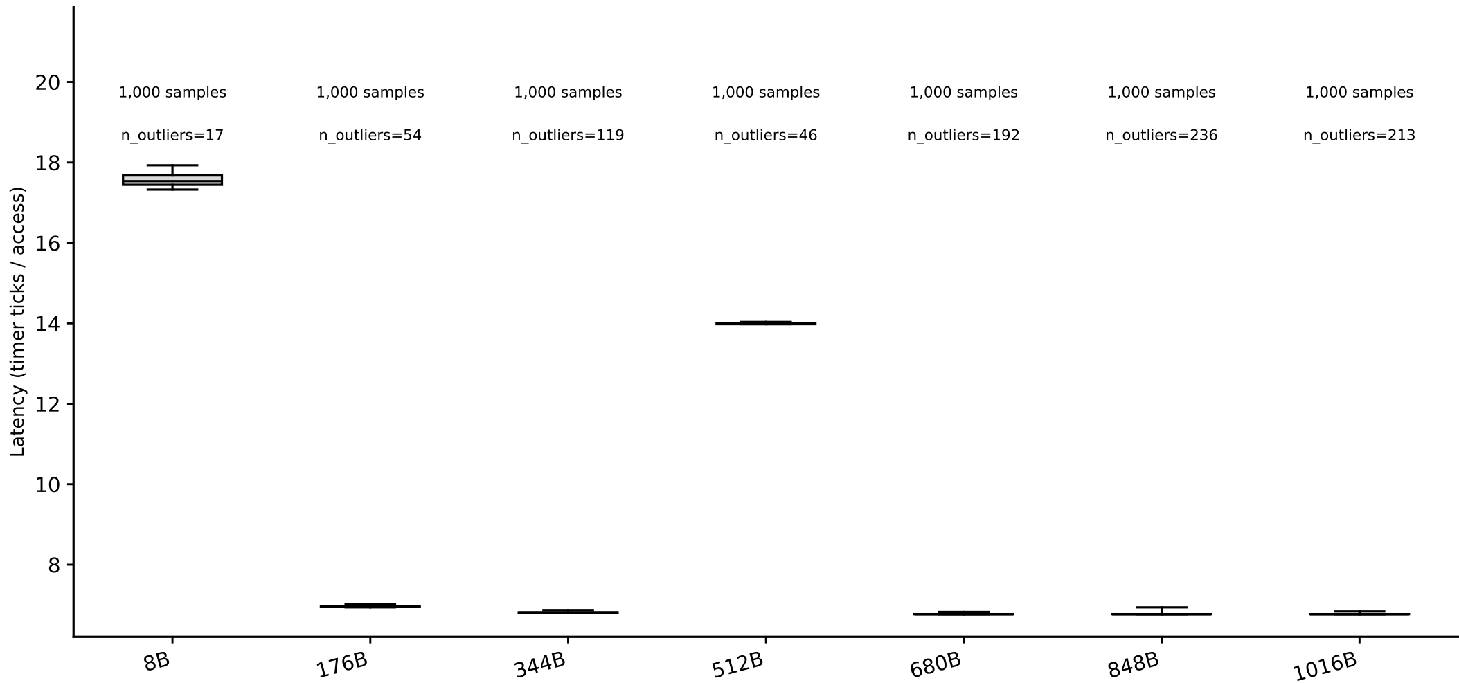
hazel_cascadelake: line-size box plots, random pattern (whiskers = p5/p95) (Phase I timing-only, level boundary=32768B, single-curve method)
