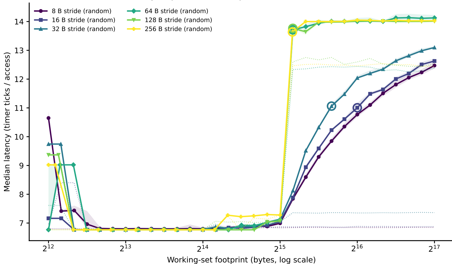
hazel_cascadelake: line-size family of curves (dependent pointer chase) (Phase I timing-only, level boundary=32768B window=[4096,131072])
