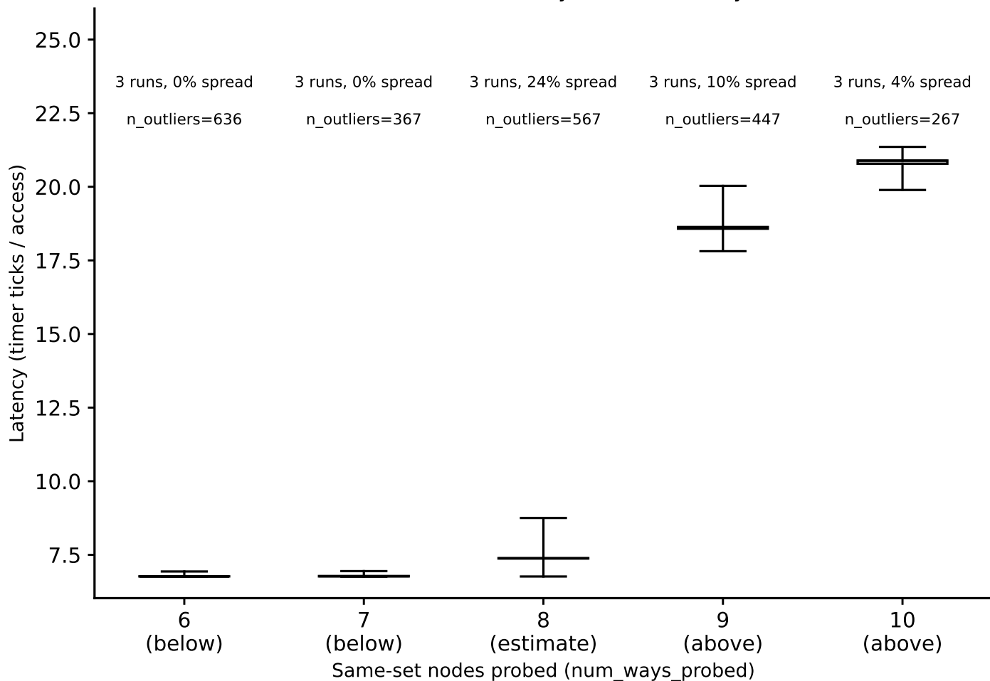
hazel_cascadelake/phase1_v2: associativity box plots, L1, random pattern (whiskers = p5/p95) (Phase I timing-only, auto pipeline) detected associativity estimate: 8-way
