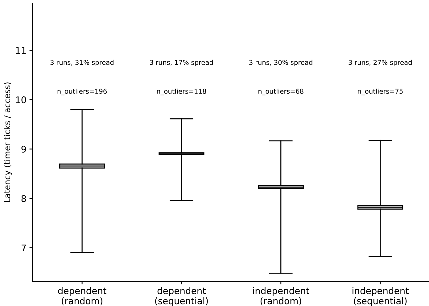
hazel_cascadelake/phase1_v2: hit-latency box plots, L1 (footprint=32 KiB) (Phase I timing-only, auto pipeline)
