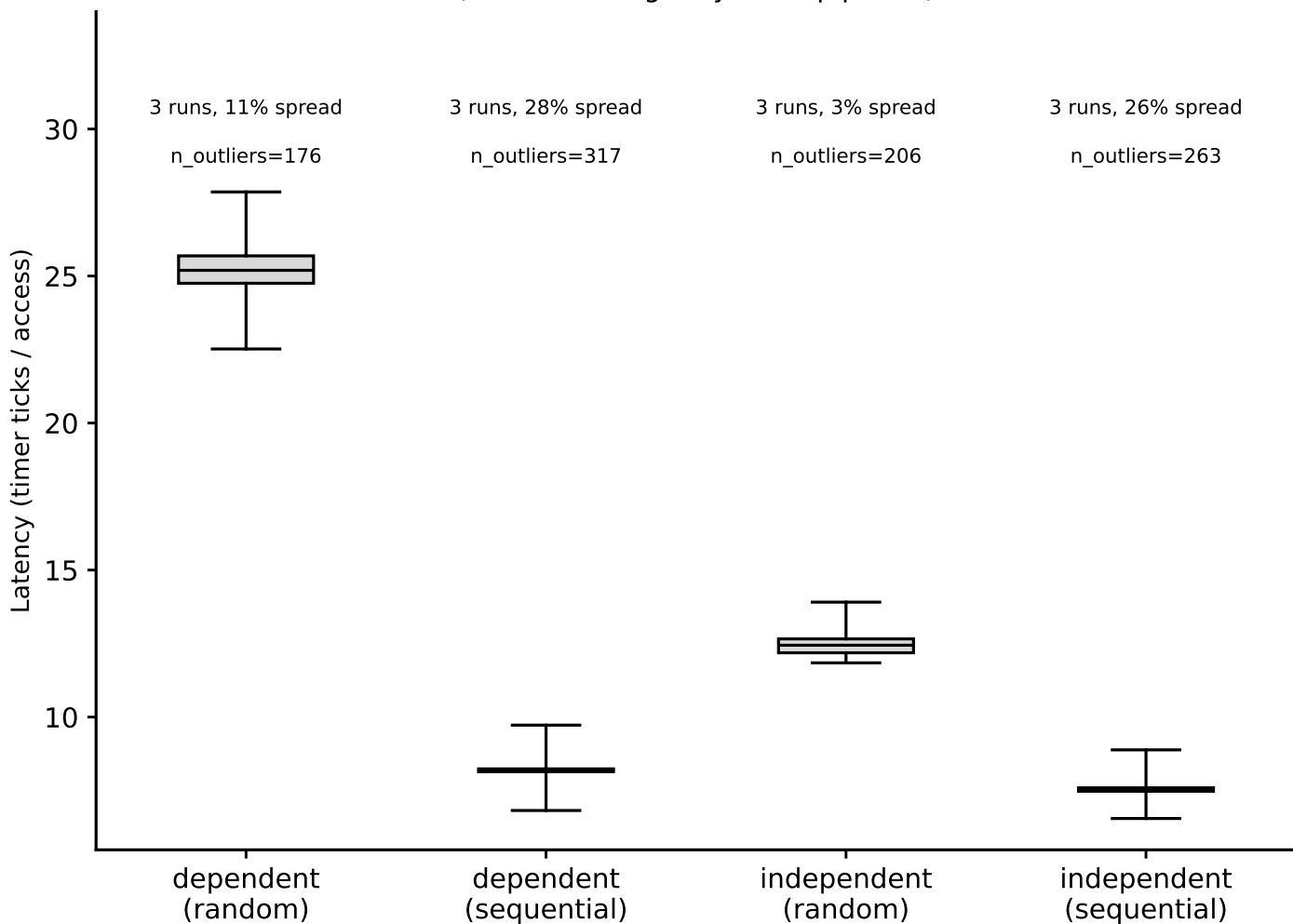
hazel_cascadelake/phase1_v2: hit-latency box plots, L2 (footprint=1 MiB) (Phase I timing-only, auto pipeline)
