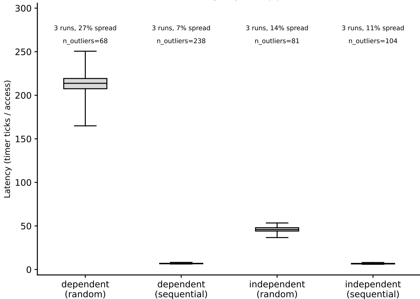
hazel_cascadelake/phase1_v2: hit-latency box plots, LLC (footprint=16 MiB) (Phase I timing-only, auto pipeline)
