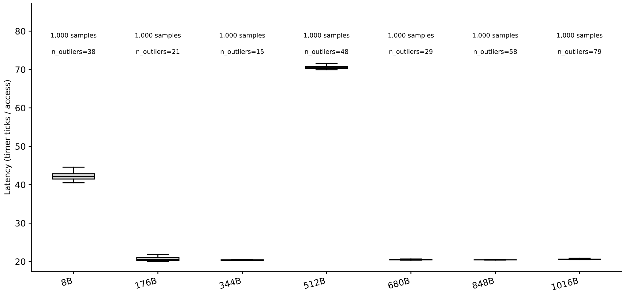
hazel_cascadelake/phase1_v2: line-size box plots, random pattern (whiskers = p5/p95) (Phase I timing-only, level boundary=1048576B, single-curve method)
