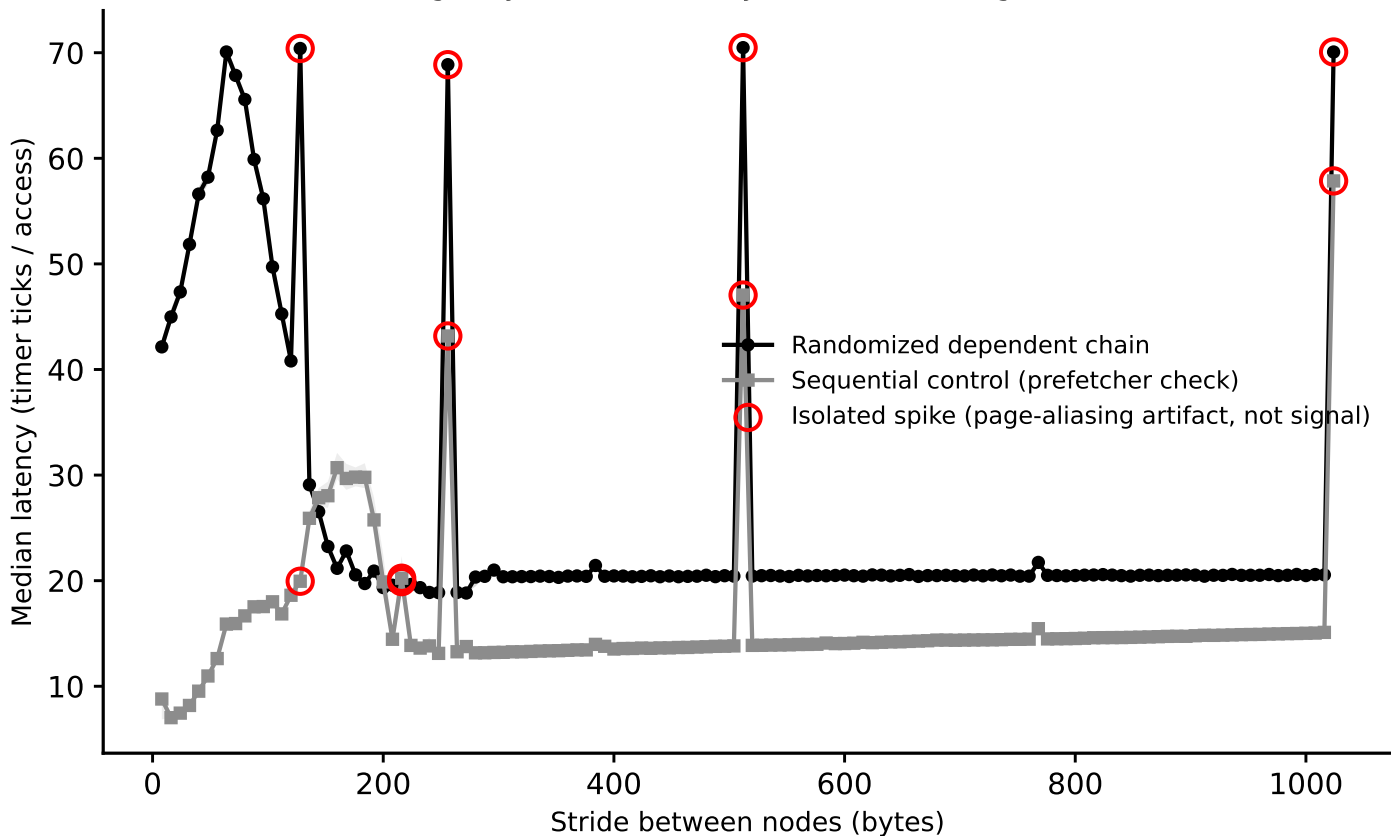
hazel_cascadelake/phase1_v2: line-size sweep (dependent pointer chase), footprint=2 MiB (Phase I timing-only, level boundary=1048576B, single-curve method)
