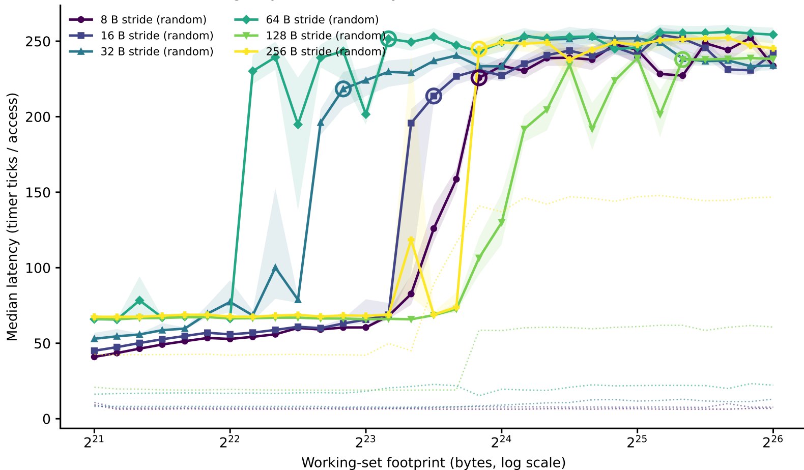
hazel_cascadelake/phase1_v2: line-size family of curves (dependent pointer chase) (Phase I timing-only, level boundary=16777216B window=[2097152,67108864])
