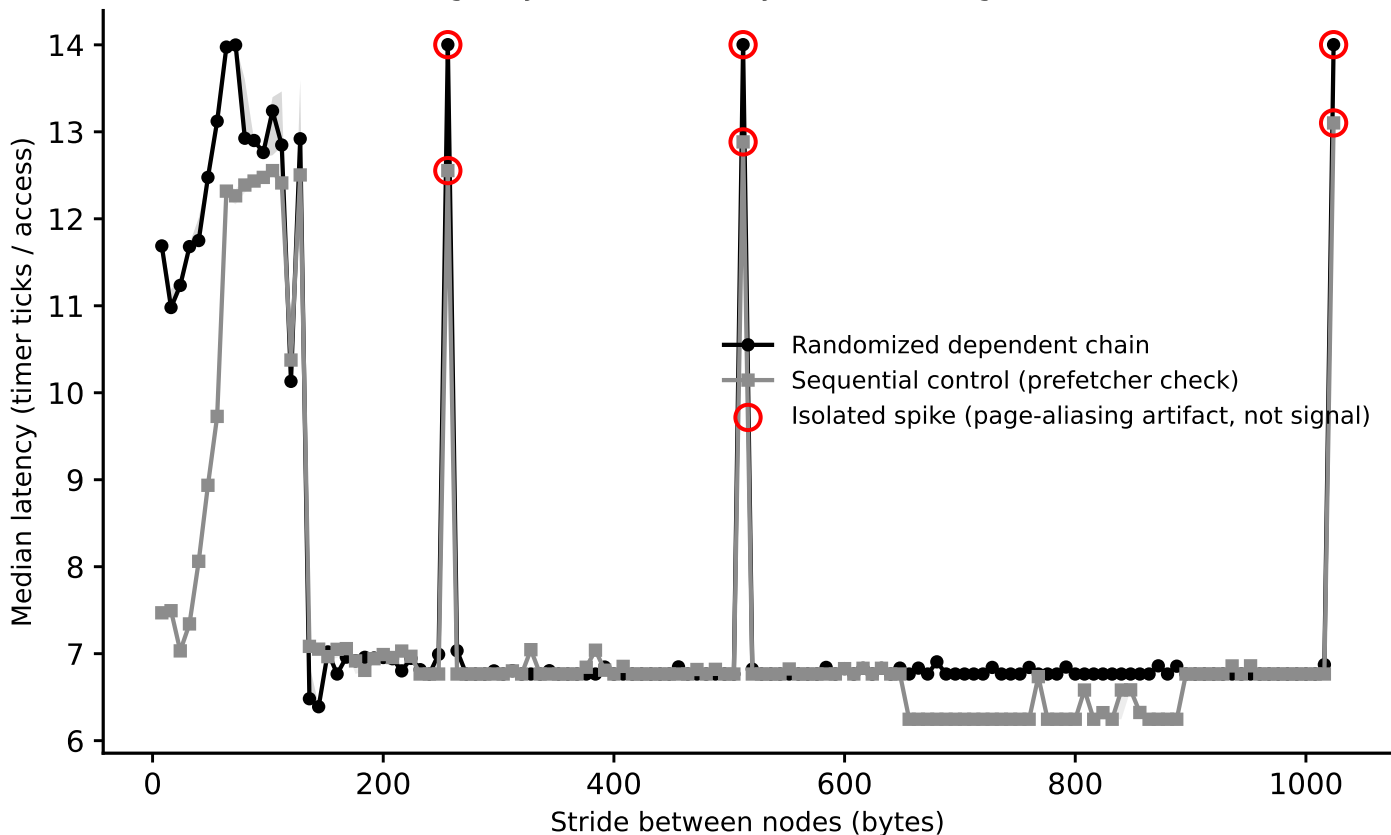
hazel_cascadelake/phase1_v2: line-size sweep (dependent pointer chase), footprint=64 KiB (Phase I timing-only, level boundary=32768B, single-curve method)
