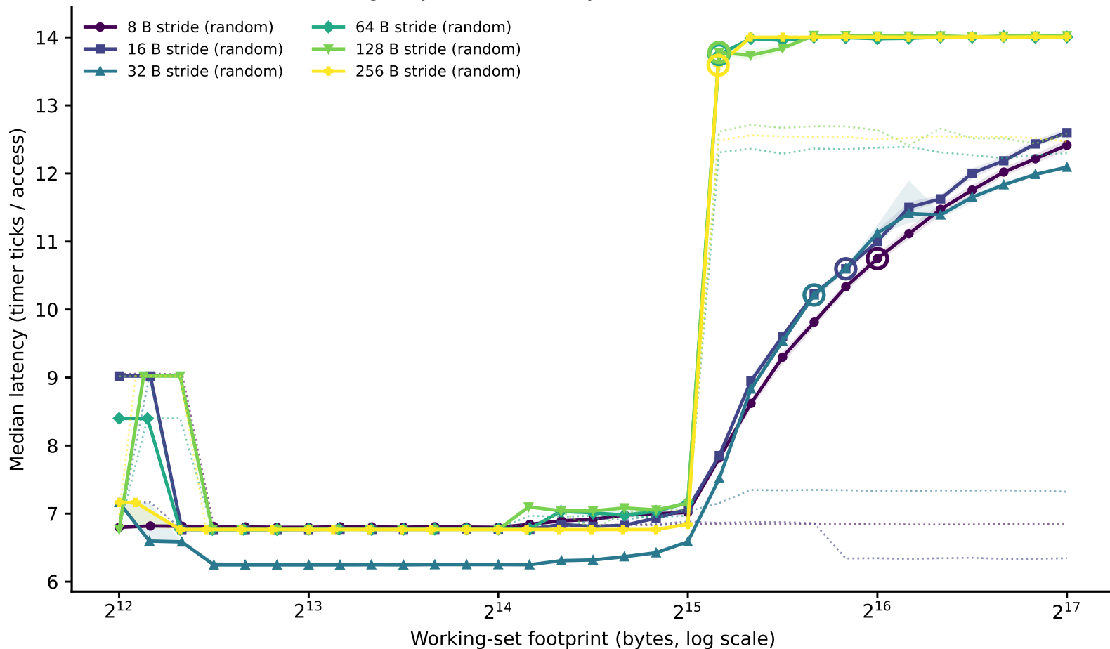
hazel_cascadelake/phase1_v2: line-size family of curves (dependent pointer chase) (Phase I timing-only, level boundary=32768B window=[4096,131072])
