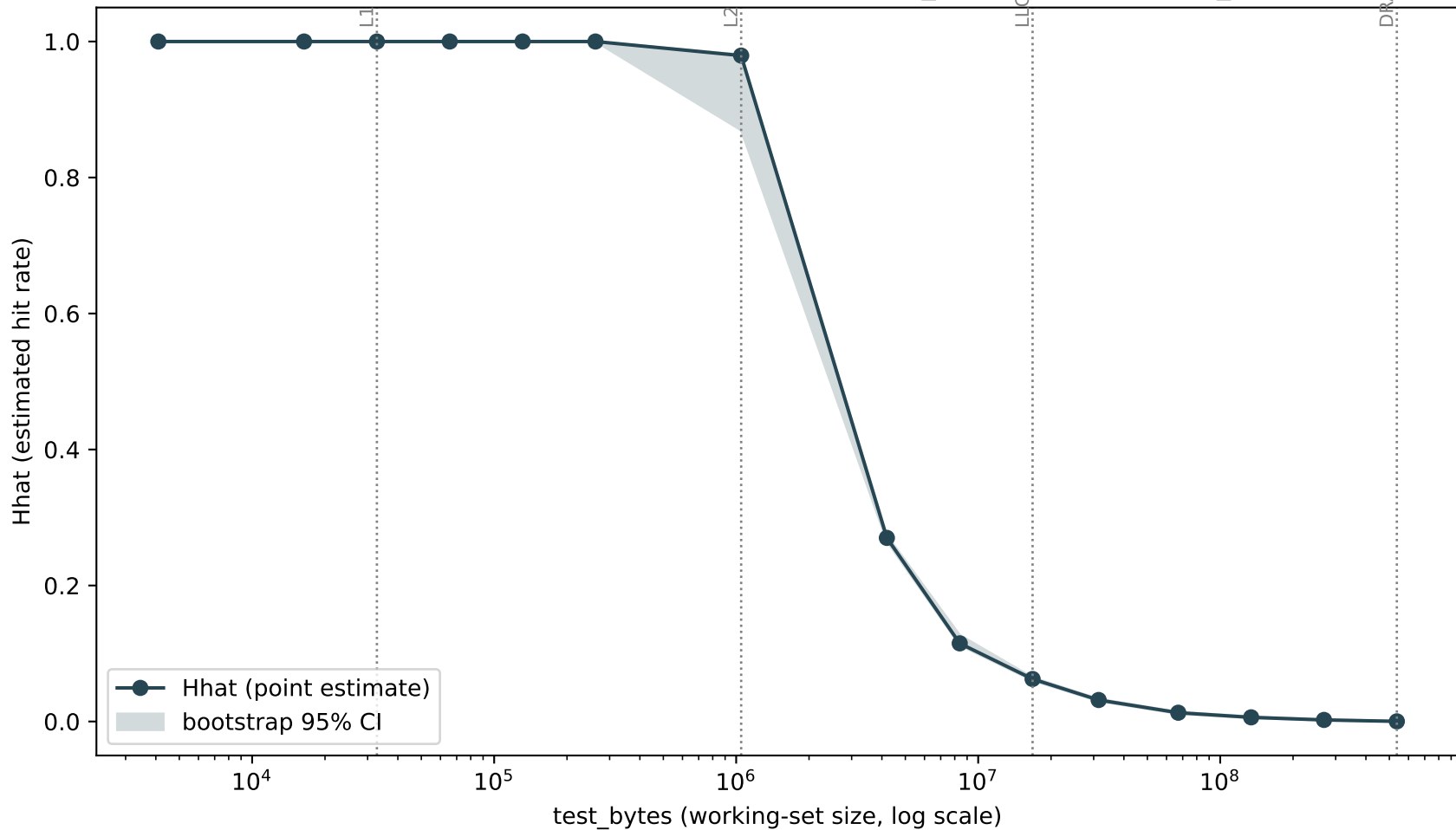
Software-only Hhat vs. working-set size (hazel_cascadelake/phase1_v2)
