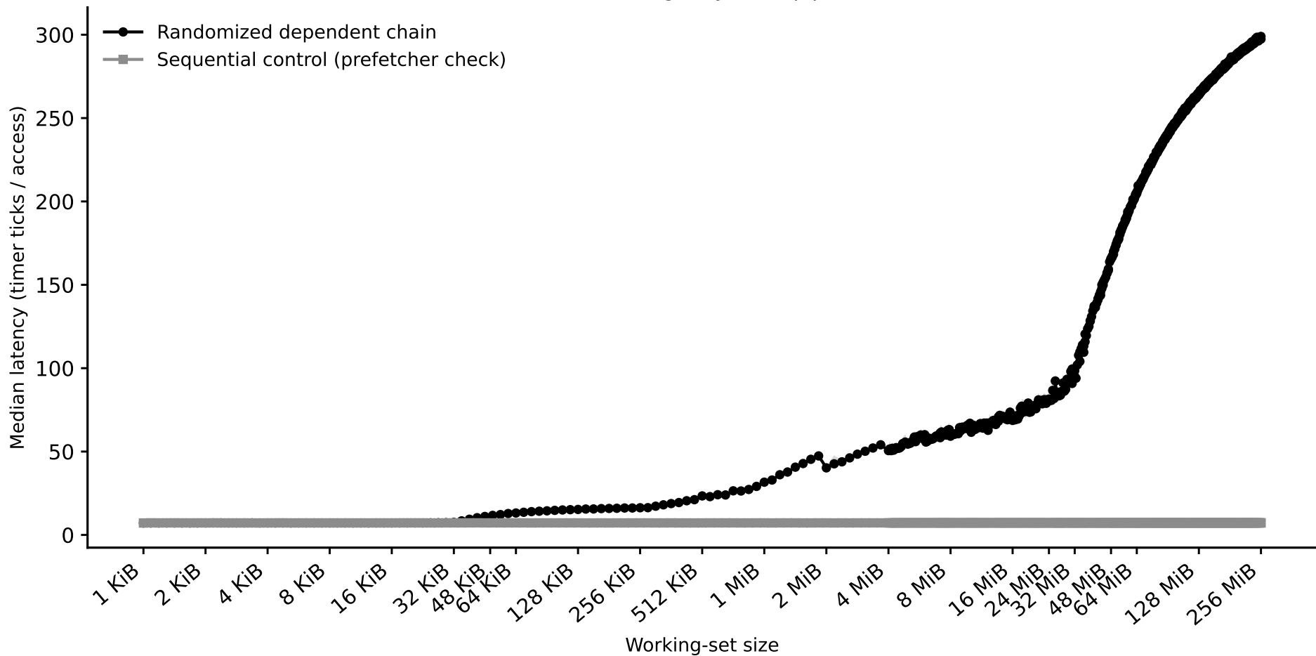
hazel_genoa: capacity sweep (dependent pointer chase) (Phase I timing-only, auto pipeline)
