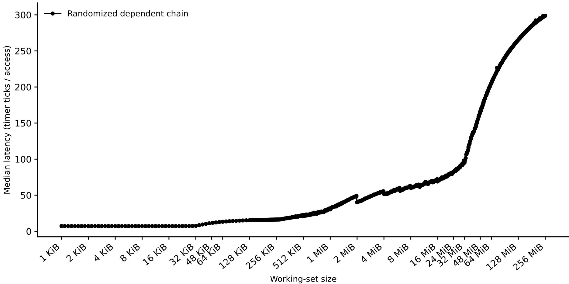
hazel_genoa/capacity_rerun: capacity sweep (dependent pointer chase) (Phase I timing-only, auto pipeline)
