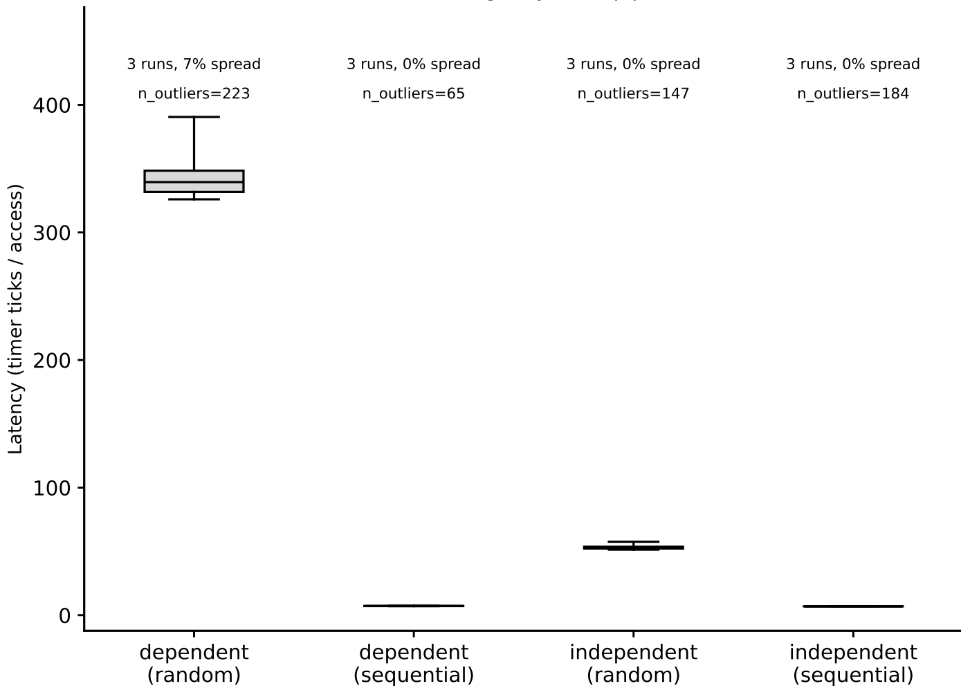
hazel_genoa: hit-latency box plots, DRAM (footprint=512 MiB) (Phase I timing-only, auto pipeline)
