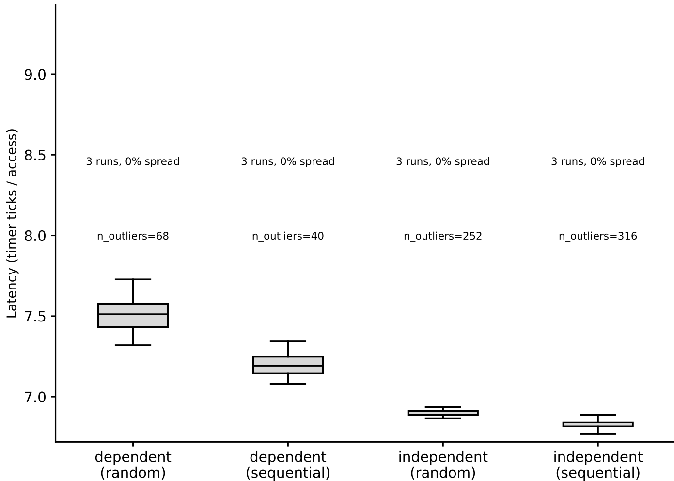
hazel_genoa: hit-latency box plots, L1 (footprint=32 KiB) (Phase I timing-only, auto pipeline)
