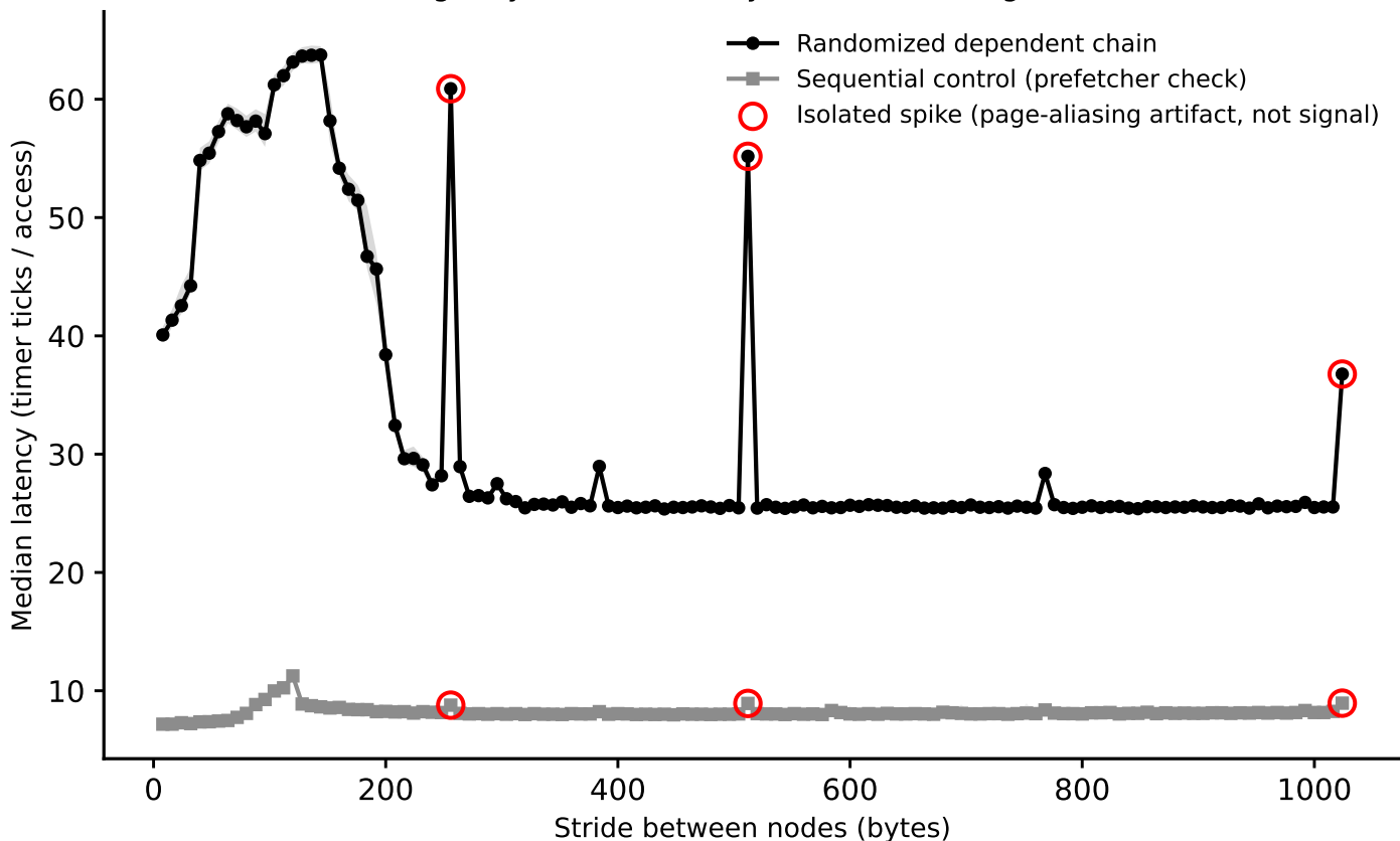
hazel_genoa: line-size sweep (dependent pointer chase), footprint=2 MiB (Phase I timing-only, level boundary=1048576B, single-curve method)
