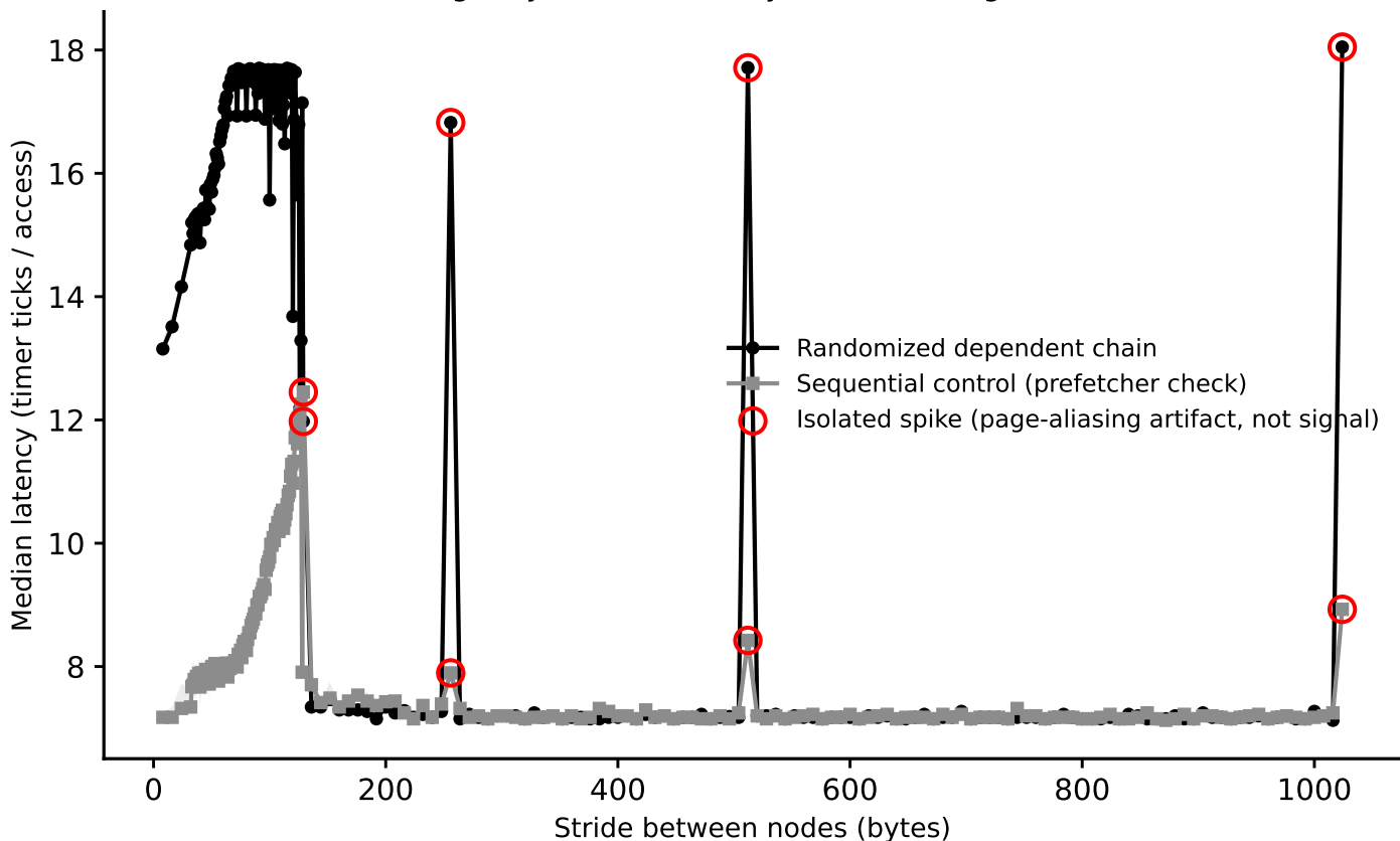
hazel_genoa: line-size sweep (dependent pointer chase), footprint=64 KiB (Phase I timing-only, level boundary=32768B, single-curve method)
