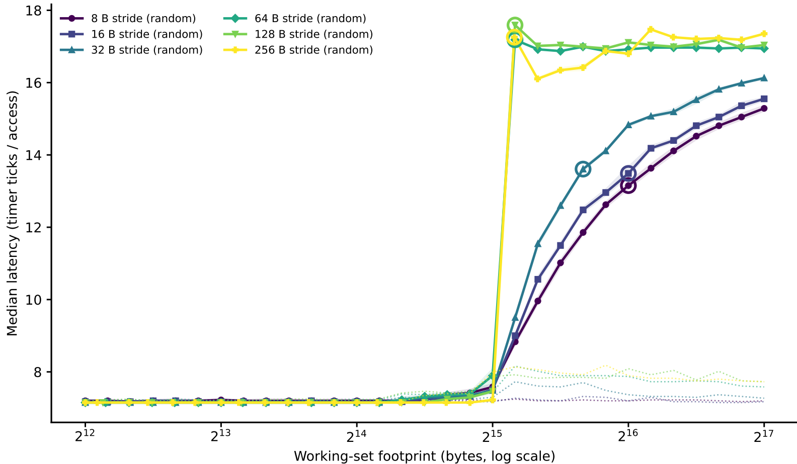
hazel_genoa: line-size family of curves (dependent pointer chase) (Phase I timing-only, level boundary=32768B window=[4096,131072])
