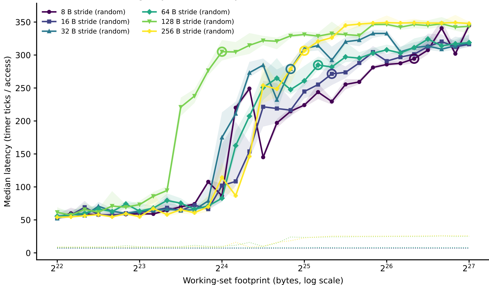
hazel_genoa: line-size family of curves (dependent pointer chase) (Phase I timing-only, level boundary=33554432B window=[4194304,134217728])
