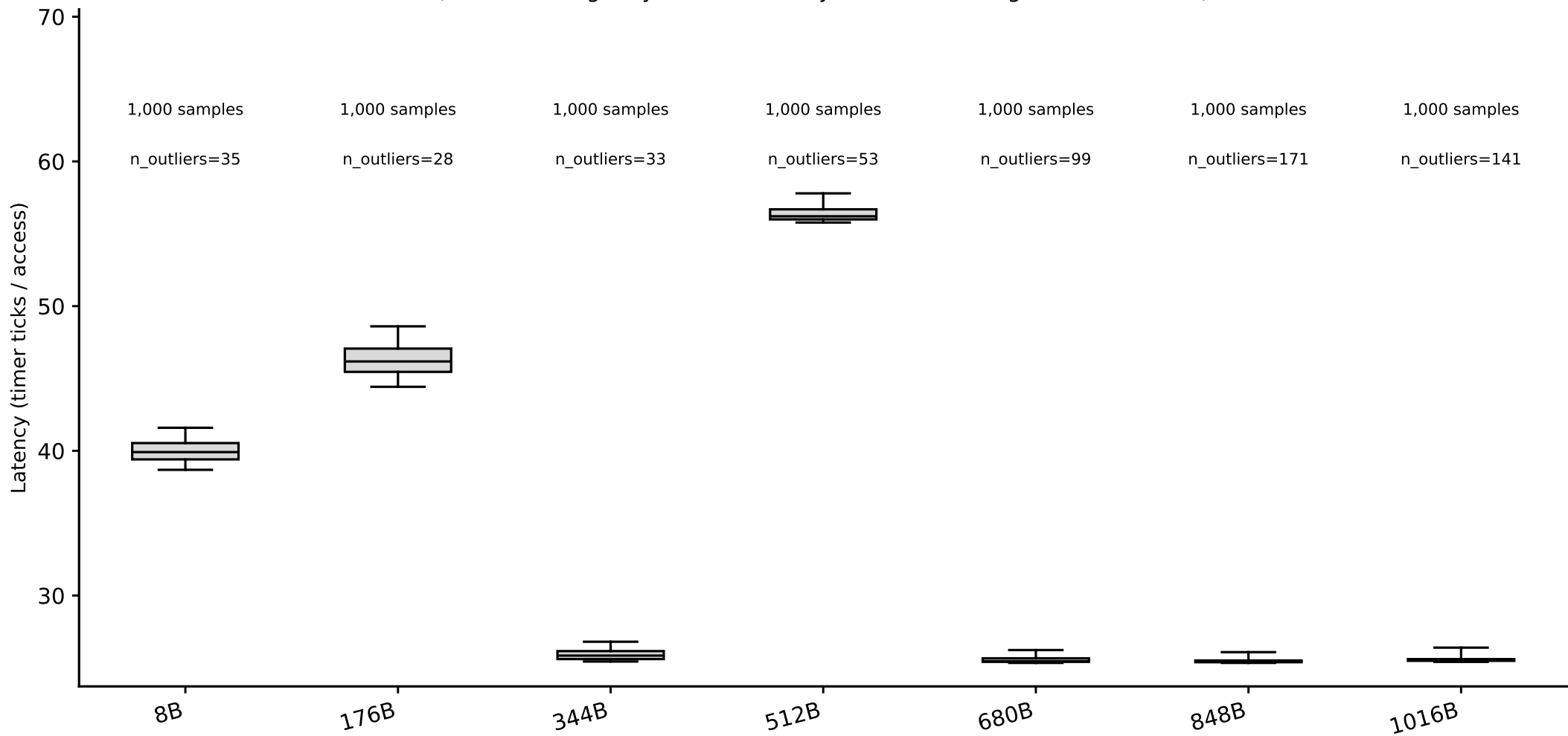
hazel_genoa/line_size_rerun: line-size box plots, random pattern (whiskers = p5/p95) (Phase I timing-only, level boundary=1048576B, single-curve method)
