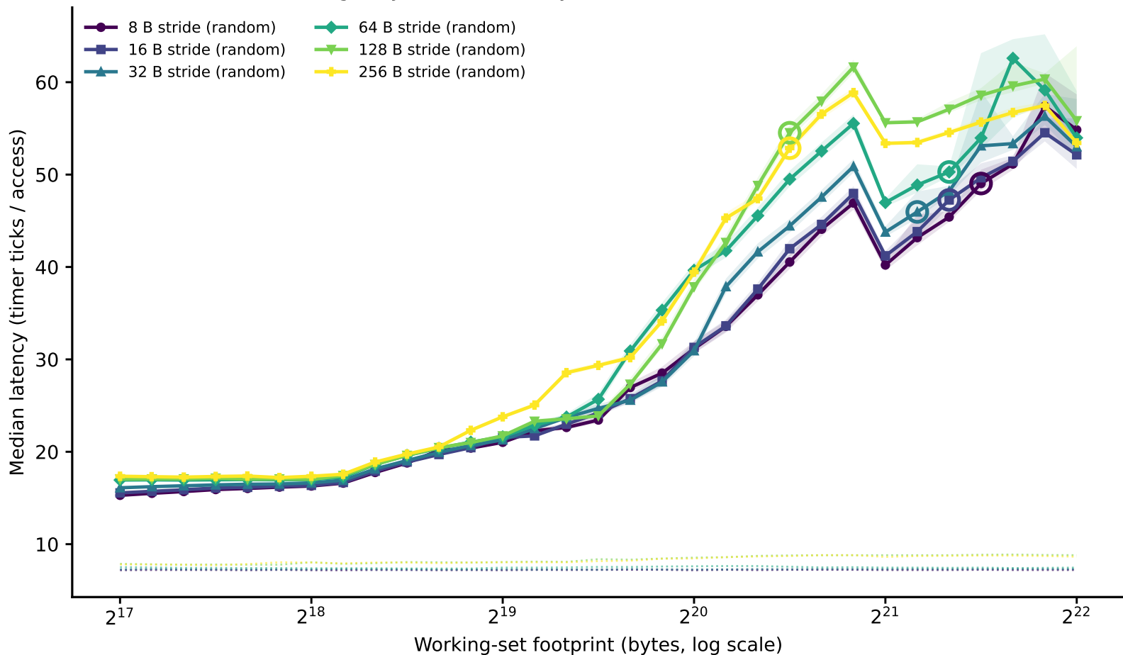
hazel_genoa/line_size_rerun: line-size family of curves (dependent pointer chase) (Phase I timing-only, level boundary=1048576B window=[131072,4194304])
