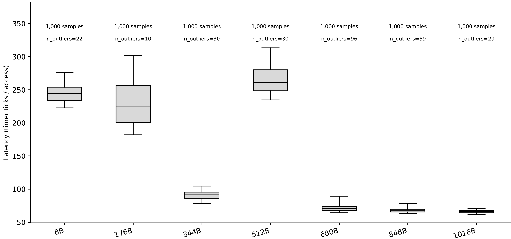
hazel_genoa/line_size_rerun: line-size box plots, random pattern (whiskers = p5/p95) (Phase I timing-only, level boundary=33554432B, single-curve method)
