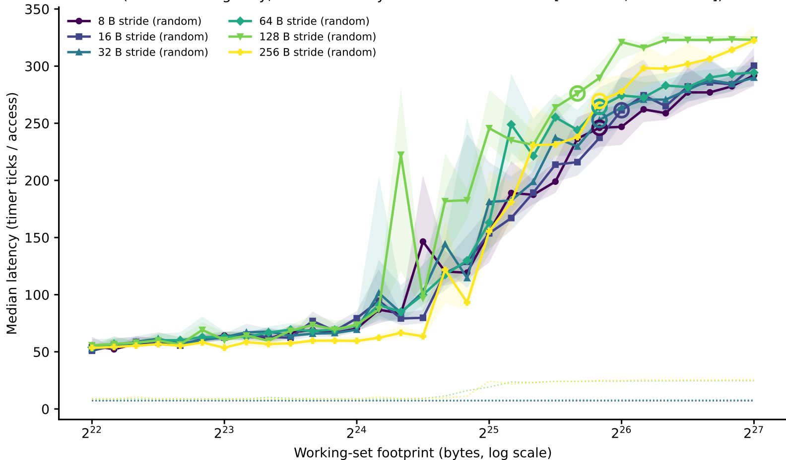
hazel_genoa/line_size_rerun: line-size family of curves (dependent pointer chase) (Phase I timing-only, level boundary=33554432B window=[4194304,134217728])
