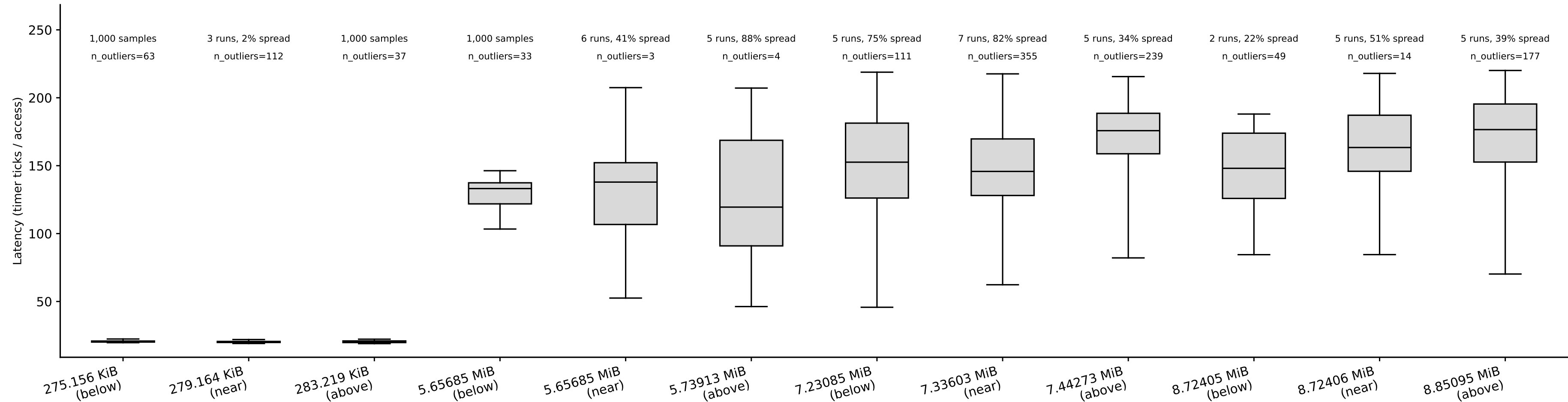
hazel_haswell/capacity_rerun: capacity box plots, random pattern (whiskers = p5/p95) (Phase I timing-only, auto pipeline) tested boundaries: 279.164 KiB, 5.65685 MiB, 7.33603 MiB, 8.72406 MiB
