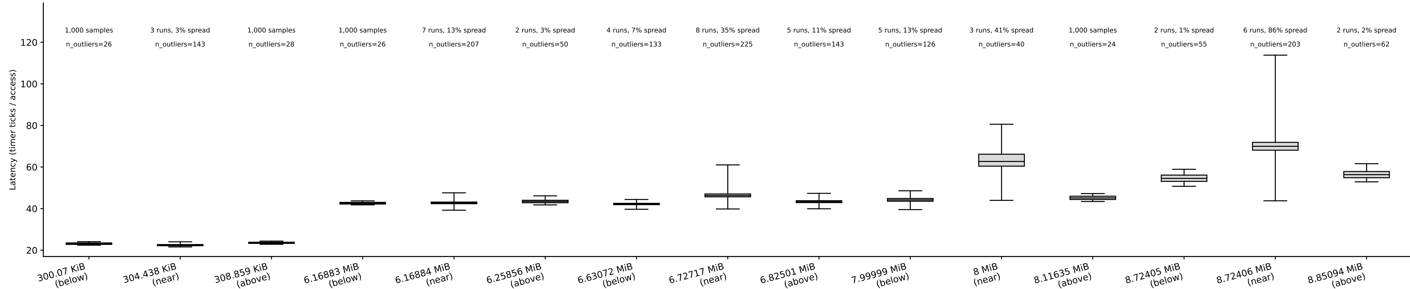
hazel_haswell/capacity_rerun2: capacity box plots, random pattern (whiskers = p5/p95) (Phase I timing-only, auto pipeline) tested boundaries: 304.438 KiB, 6.16884 MiB, 6.72717 MiB, 8 MiB, 8.72406 MiB
