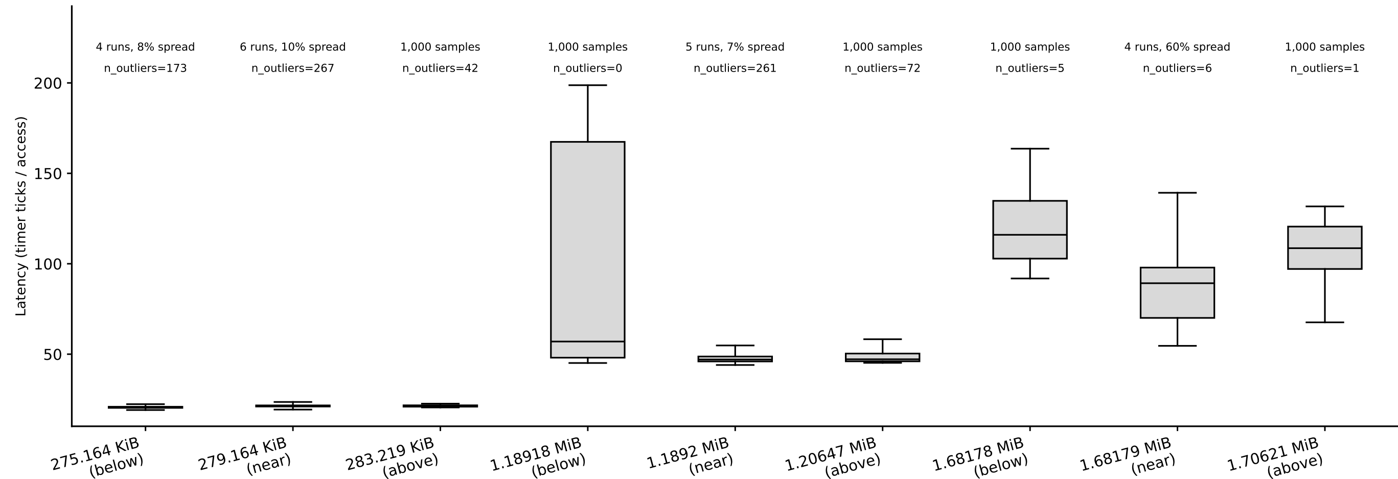
hazel_haswell/capacity_rerun3: capacity box plots, random pattern (whiskers = p5/p95) (Phase I timing-only, auto pipeline) tested boundaries: 279.164 KiB, 1.1892 MiB, 1.68179 MiB
