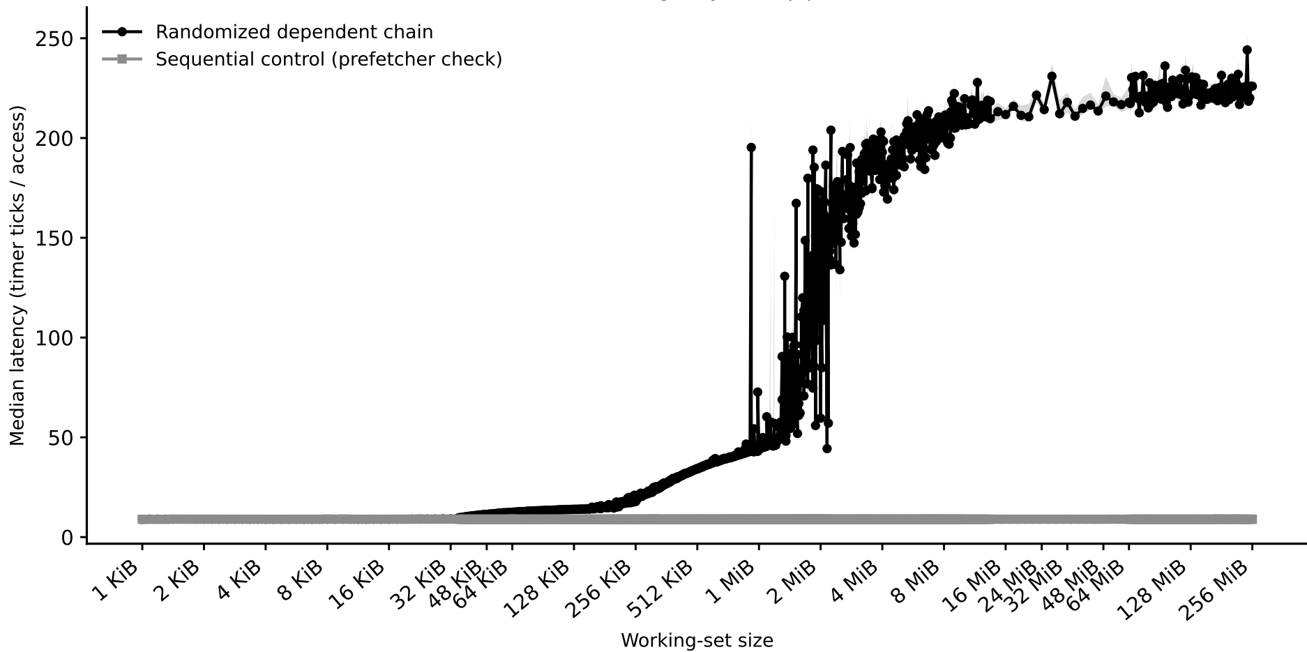
hazel_haswell/capacity_rerun3: capacity sweep (dependent pointer chase) (Phase I timing-only, auto pipeline)
