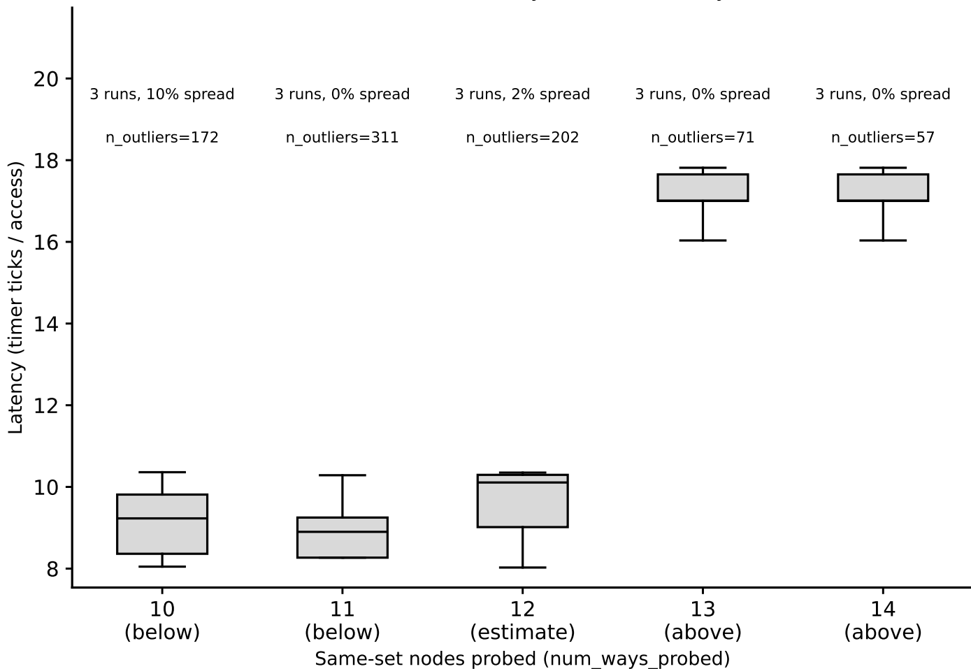
hazel_icelake_6326: associativity box plots, L2, random pattern (whiskers = p5/p95) (Phase I timing-only, auto pipeline) detected associativity estimate: 12-way
