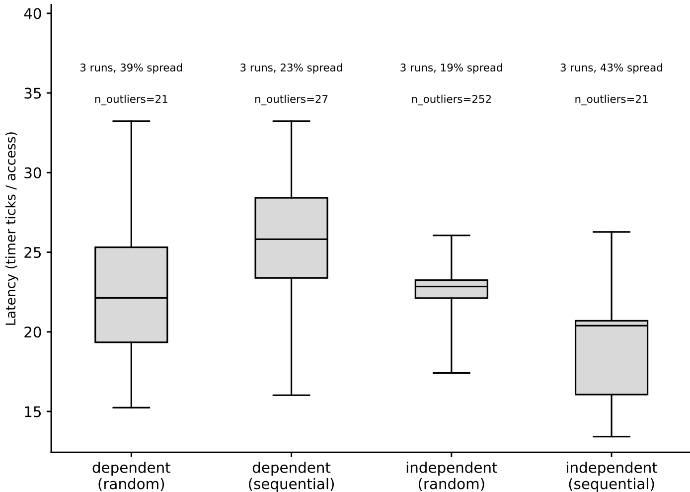
hazel_icelake_6326: hit-latency box plots, L1 (footprint=32 KiB) (Phase I timing-only, auto pipeline)
