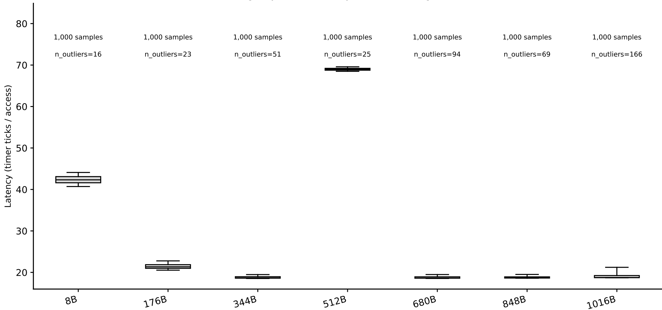
hazel_icelake_6326: line-size box plots, random pattern (whiskers = p5/p95) (Phase I timing-only, level boundary=1310720B, single-curve method)
