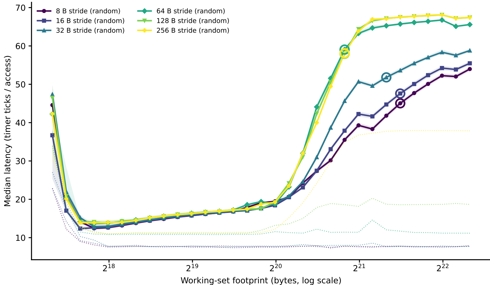
hazel_icelake_6326: line-size family of curves (dependent pointer chase) (Phase I timing-only, level boundary=1310720B window=[163840,5242880])
