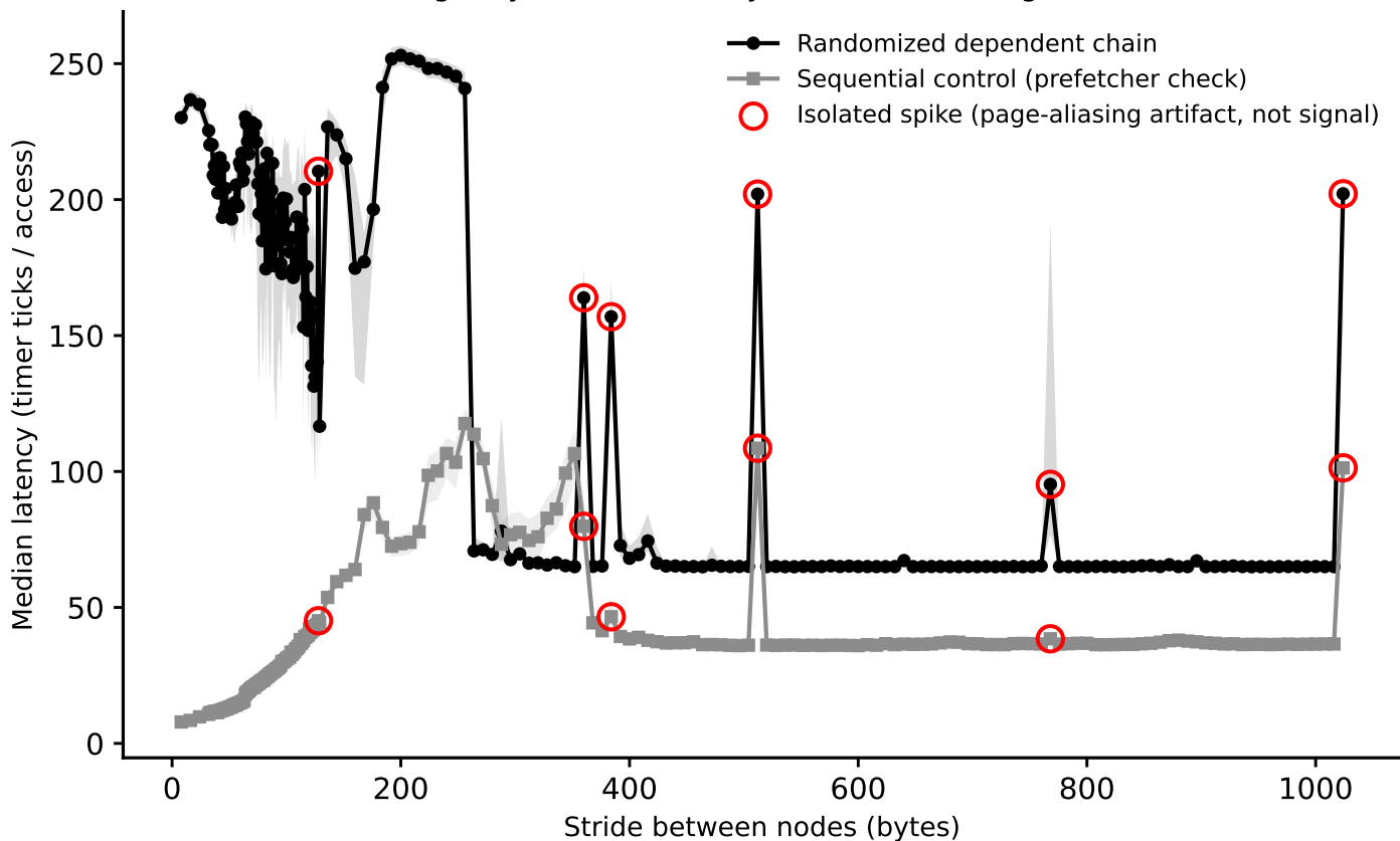
hazel_icelake_6326: line-size sweep (dependent pointer chase), footprint=49.3507 MiB (Phase I timing-only, level boundary=25874000B, single-curve method)
