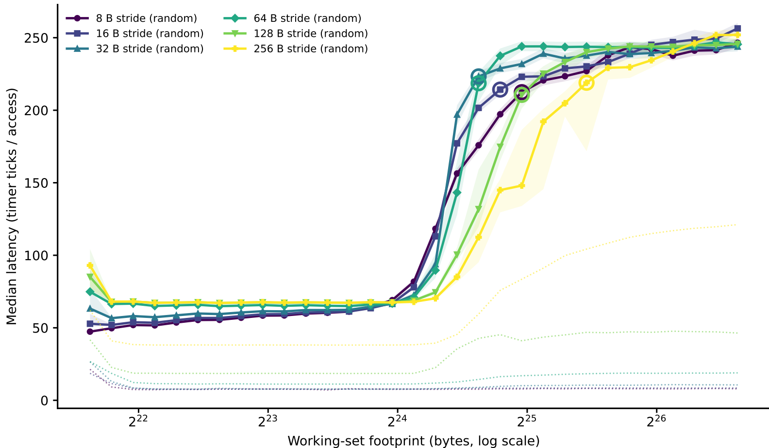
hazel_icelake_6326: line-size family of curves (dependent pointer chase) (Phase I timing-only, level boundary=25874000B window=[3234250,103496000])
