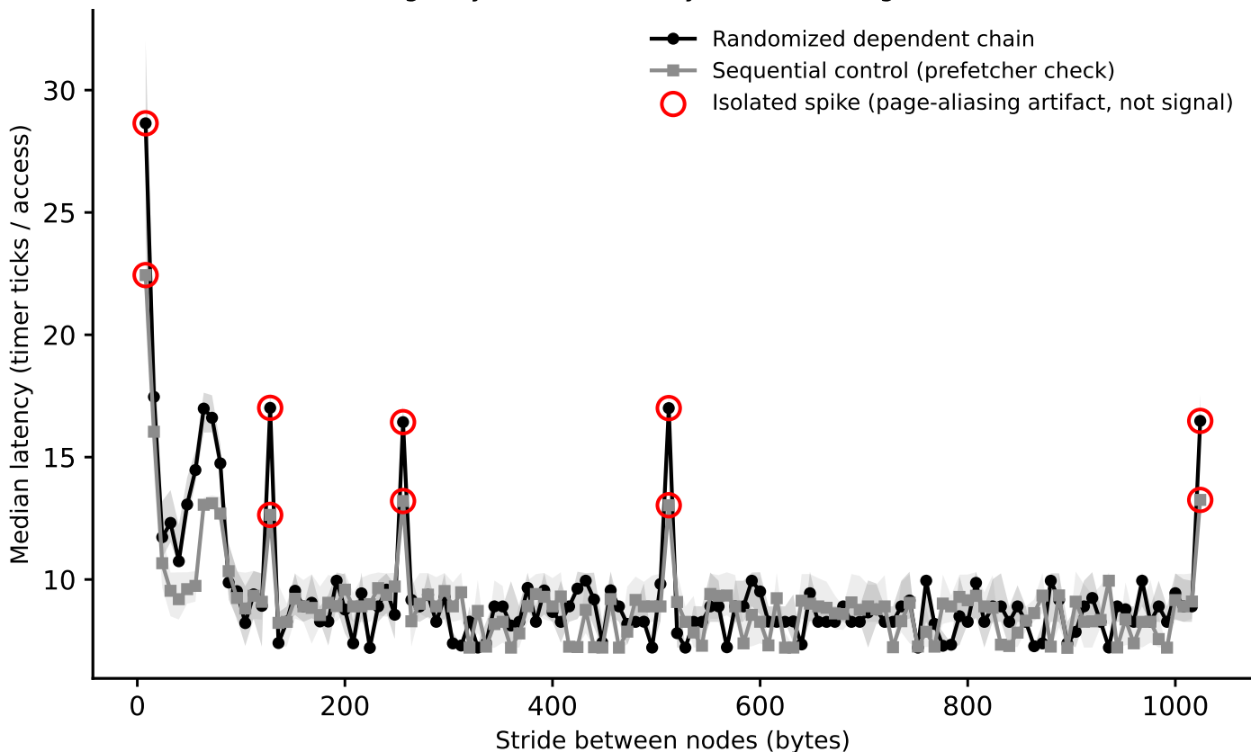
hazel_icelake_6326: line-size sweep (dependent pointer chase), footprint=64 KiB (Phase I timing-only, level boundary=32768B, single-curve method)
